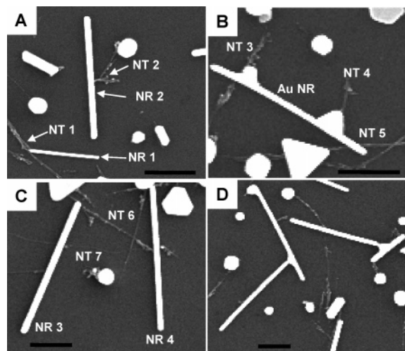
Figure 1. SEM images of Au NR/SWCNT heterojunctions. (A) NRs attached to the side wall and end of nanotubes from Au MPCs grown in one (NR 1) or two (NR 2) directions. (B) Au NR attached to three different SWCNT bundles (NT 3, NT 4, and NT 5). (C) Two Au NRs (NR 3 and NR 4) attached to the same bundle of SWCNTs (NT 6 and NT 7). (D) Connection between six NRs and at least eight different SWCNT bundles. Scale bars are 250 nm.
