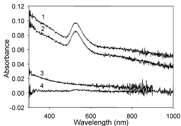
Figure 2. Visible spectra of (1) glass/APTES/SWCNT/Au MPCs (15 min), (2) glass/APTES/SWCNT/Au MPCs (10 min), (3) glass/APTES/SWCNTs (2 days), and (4) glass/APTES/Au MPCs (15 min) placed in growth solution for 1 h.
